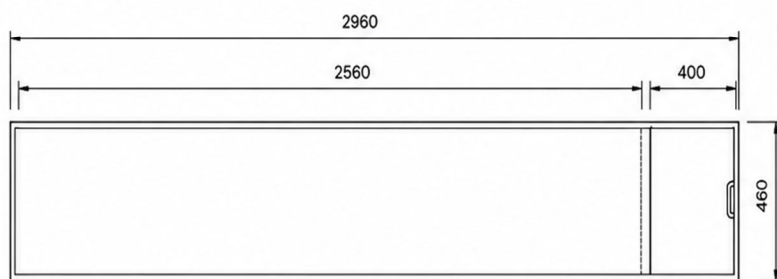
PLAN (TOP VIEW)
