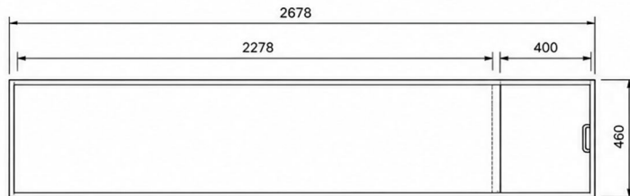
PLAN (TOP VIEW)
