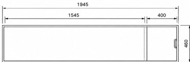
PLAN (TOP VIEW)
