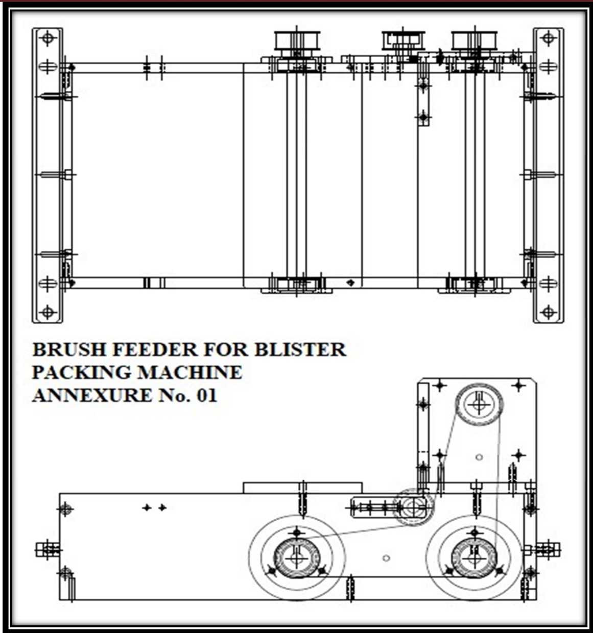
ROTARY BRUSH FEEDER FOR BLISTER PACKING MACHINE 240
